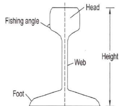
FLAT-FOOTED RAIL
