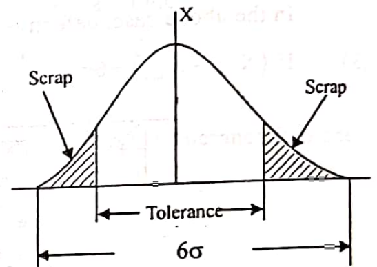
Fig.2.20 Statistical limits outside tolerance limits.
