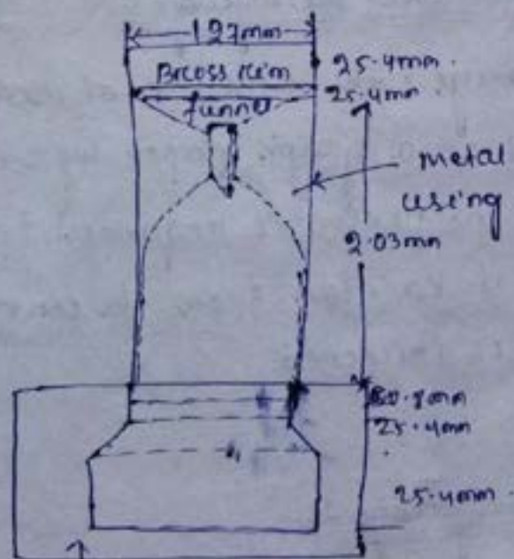
c.c foundation block 600 x 600 x 600mm Simon's rain gauge
