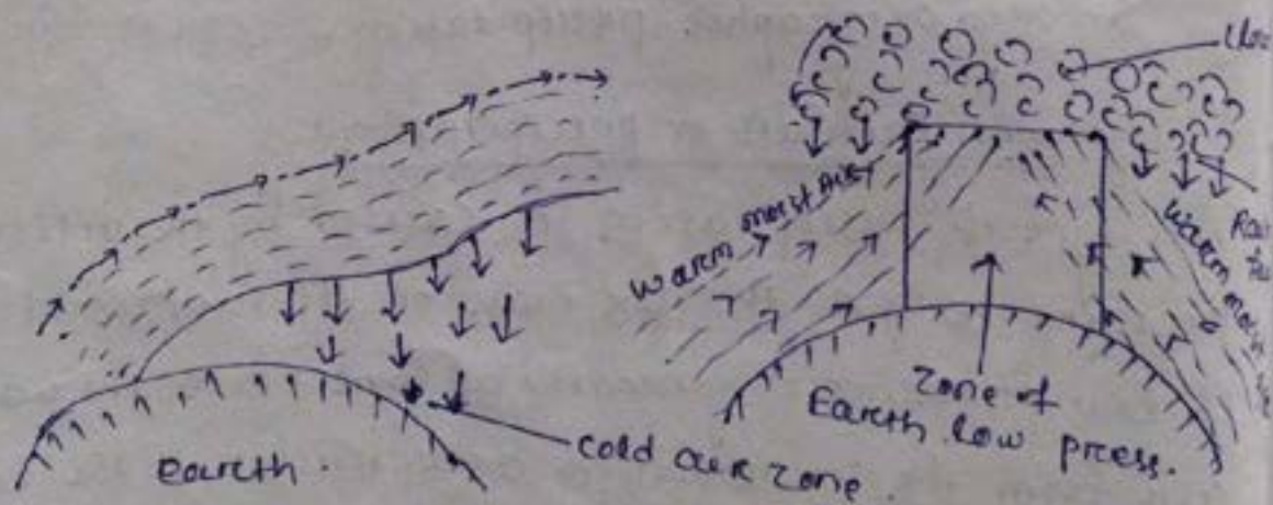
Nonfrontal precipitation
