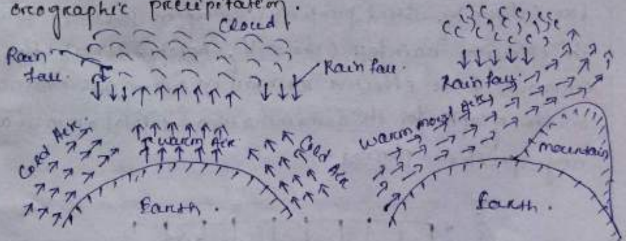
Convective Rainfall.
