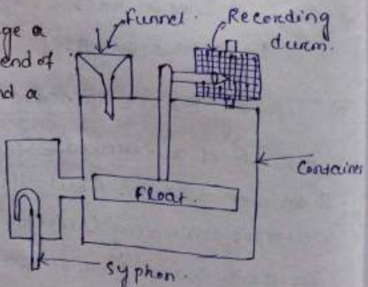
Float Type Rain gauge.
