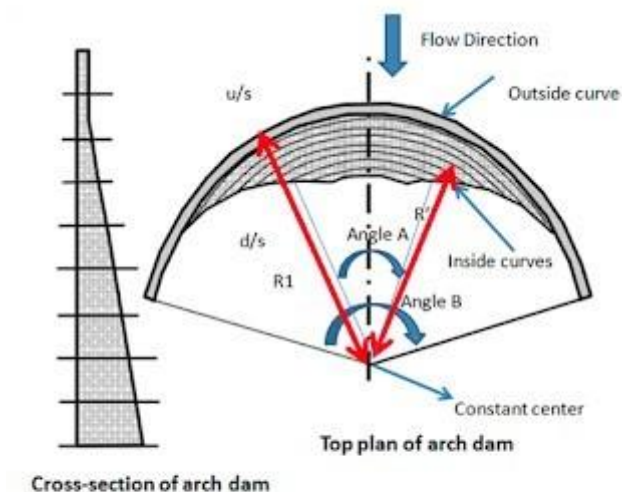
Constant Radii Arch Dam Best suited for U-Shaped Valley
