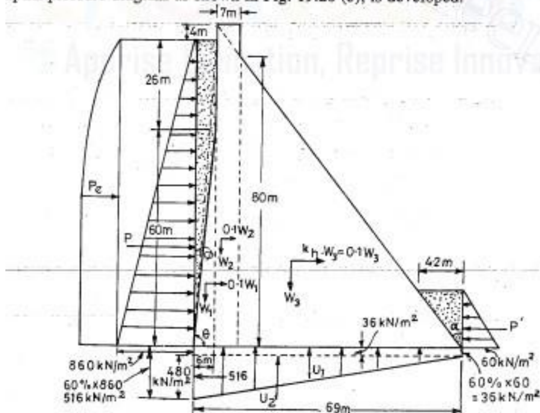
Fig. 19.20 (c) Reservoir full case
