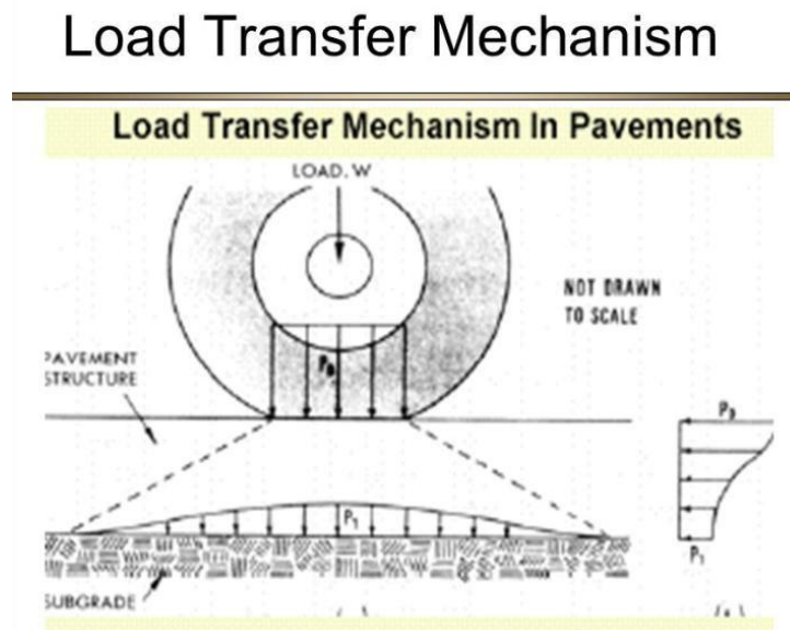
Figure 4 : Load transfer in rigid pavement
